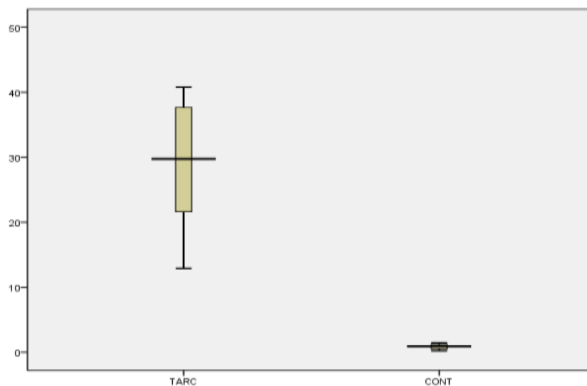
Figure 1: Boxplot shows comparison between RSV-A-induced TARC with control (RSV-A negative).
