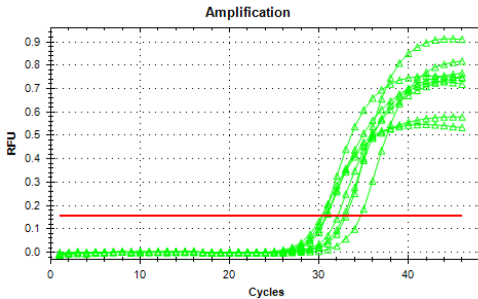
Figure 4: Real-Time PCR amplification plot for MDC gene in (RSV-A) positive samples.
