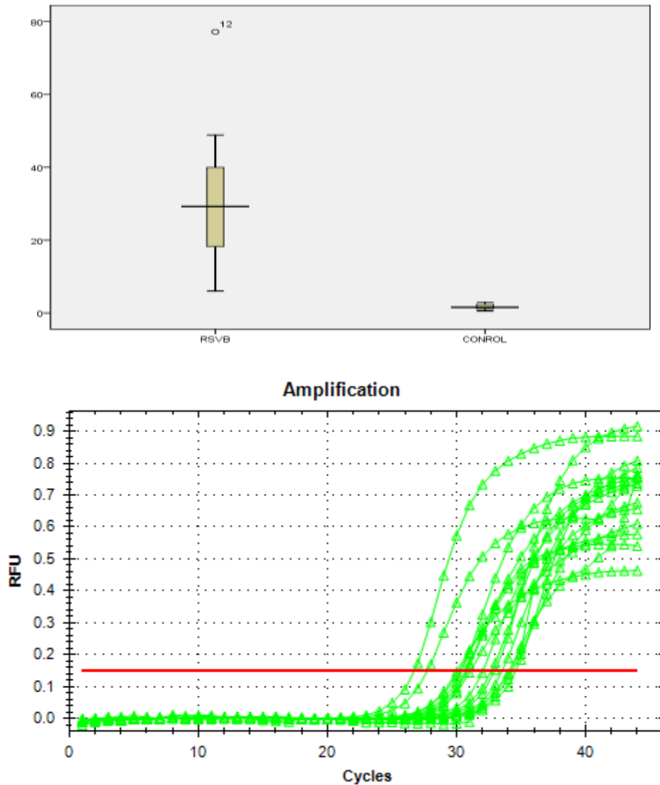
Figure 5: Real-Time PCR amplification plot for MDC gene in (RSV-B) positive samples
