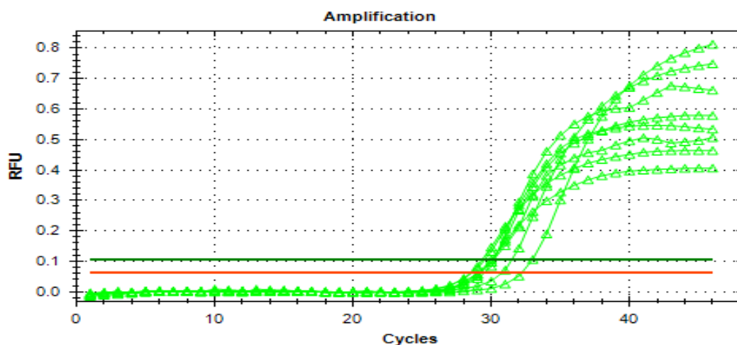
Figure 2: Amplification plot of RT-PCR for TARC gene in (RSV-A) (positive samples).
