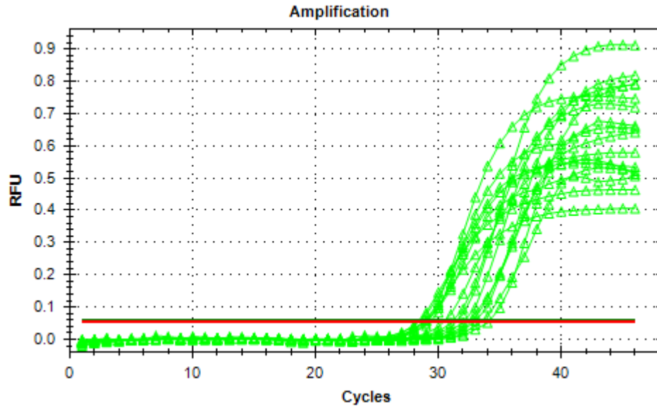
Figure 3: Real-Time PCR amplification plot for TARC gene in (RSV-B) positive patient sample
